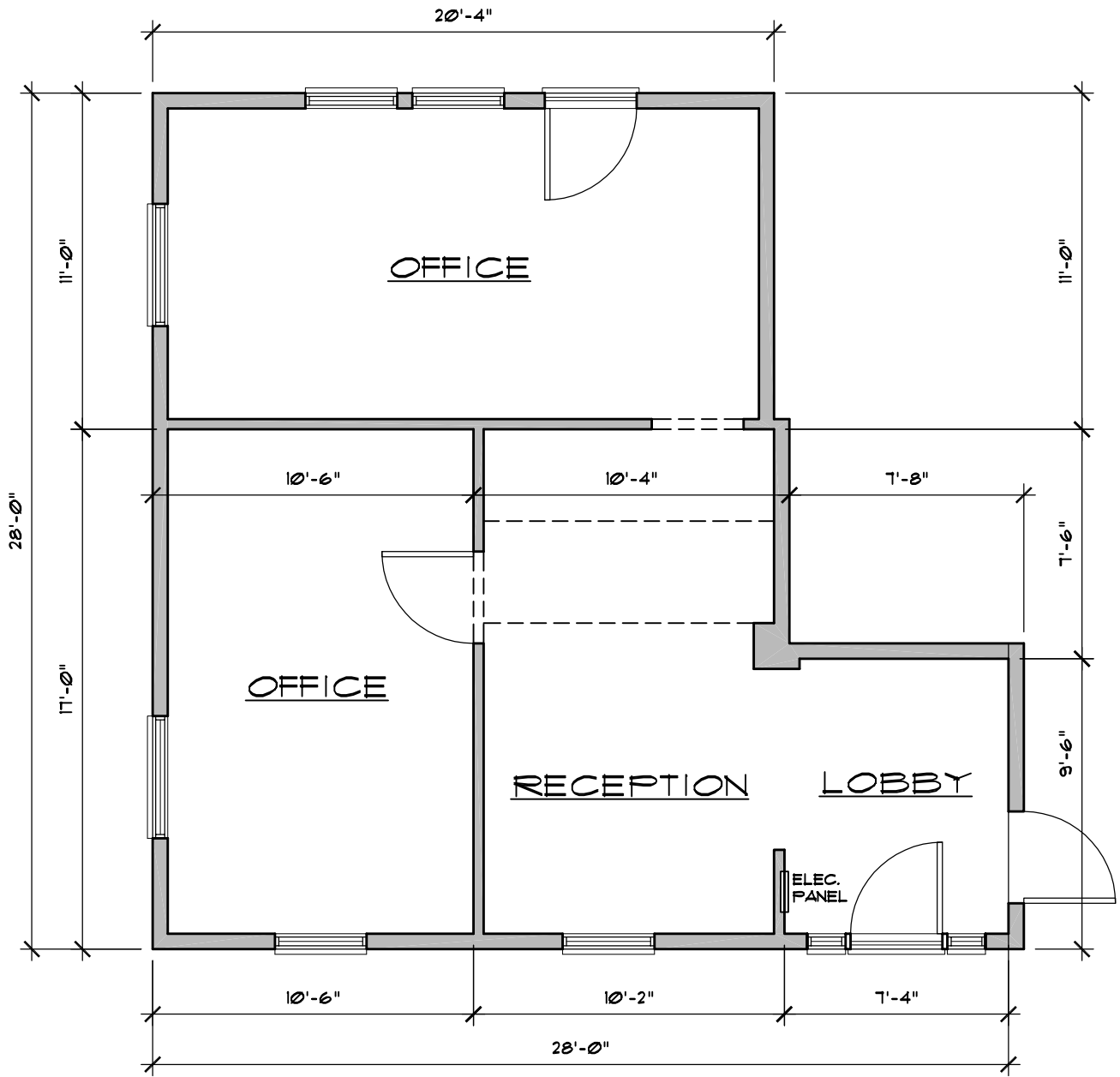
FLOOR PLAN 674 s.f. 827-C ALDER CREEK DRIVE
